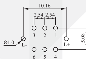
P.C.B. Mounting Holes
